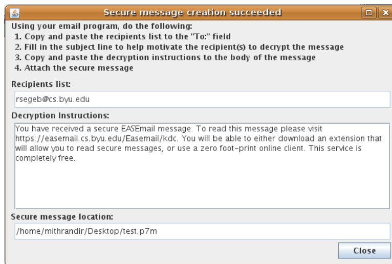
Figure 4.7: Java applet secure message creation information screen
